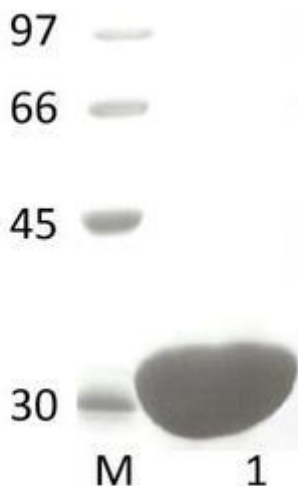
Figure 1. SDS-PAGE analysis of CmCel5B (GH5) was conducted in (Lane 1), employing a 14% polyacrylamide gel. The enzyme exhibits a band corresponding to a molecular weight of approximately 33,99 kDa. Lane M contains a Protein Marker for reference.
