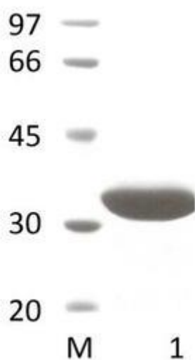
Figure 1. SDS-PAGE analysis of CtCel5E (GH5) was conducted in (Lane 1), employing a 14% polyacrylamide gel. The enzyme exhibits a band corresponding to a molecular weight of approximately 37,27 kDa. Lane M contains a Protein Marker for reference.
