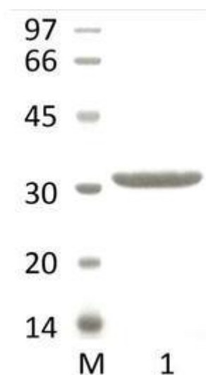
Figure 1. SDS-PAGE analysis of CtLic26A (GH26) was conducted in (Lane 1), employing a 14% polyacrylamide gel. The enzyme exhibits a band corresponding to a molecular weight of approximately 32,51 kDa. Lane M contains a Protein Marker for reference.
