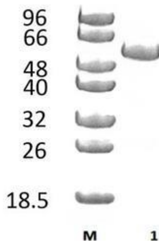
Figure 1. SDS-PAGE analysis of GFP-CBM9 was conducted in (Lane 1), employing a 14% polyacrylamide gel. The enzyme exhibits a band corresponding to a molecular weight of approximately 50,62 kDa. Lane M contains a Protein Marker for reference.
