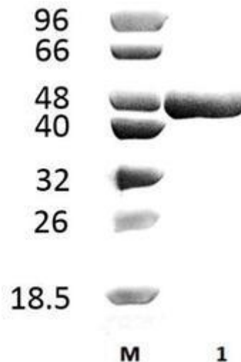
Figure 1. SDS-PAGE analysis of GFP-CBM3 was conducted in (Lane 1), employing a 14% polyacrylamide gel. The enzyme exhibits a band corresponding to a molecular weight of approximately 46,29 kDa. Lane M contains a Protein Marker for reference.
