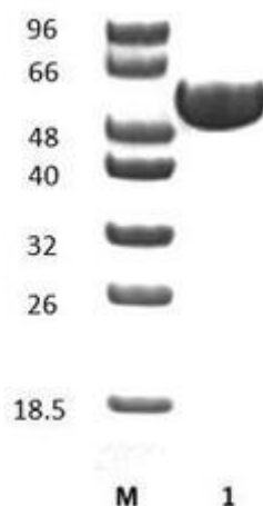
Figure 1. SDS-PAGE analysis of BsPbg1C (GH1) was conducted in (Lane 1), employing a 14% polyacrylamide gel. The enzyme exhibits a band corresponding to a molecular weight of approximately 57,19 kDa. Lane M contains a Protein Marker for reference.
