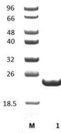
Figure 1. SDS-PAGE analysis of BsXyn11A (GH11) was conducted in (Lane 1), employing a 14% polyacrylamide gel. The enzyme exhibits a band corresponding to a molecular weight of approximately 22,47 kDa. Lane M contains a Protein Marker for reference.
