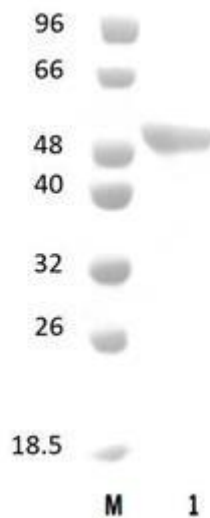
Figure 1. SDS-PAGE analysis of BsPgx4A (GH4) was conducted in (Lane 1), employing a 14% polyacrylamide gel. The enzyme exhibits a band corresponding to a molecular weight of approximately 51,54 kDa. Lane M contains a Protein Marker for reference.
