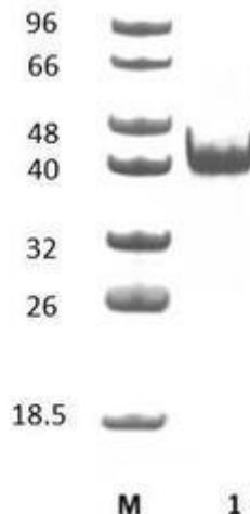
Figure 1. SDS-PAGE analysis of BtAbf43C (GH43) was conducted in (Lane 1), employing a 14% polyacrylamide gel. The enzyme exhibits a band corresponding to a molecular weight of approximately 40,45 kDa. Lane M contains a Protein Marker for reference.
