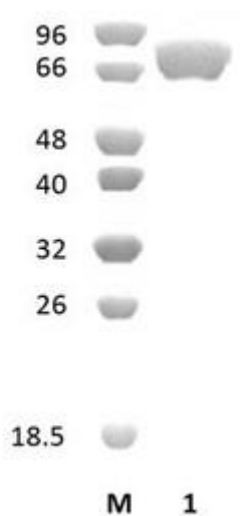
Figure 1. SDS-PAGE analysis of BtMns92D (GH92) was conducted in (Lane 1), employing a 14% polyacrylamide gel. The enzyme exhibits a band corresponding to a molecular weight of approximately 86,17 kDa. Lane M contains a Protein Marker for reference.
