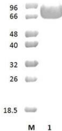
Figure 1. SDS-PAGE analysis of BtMns92E (GH92) was conducted in (Lane 1), employing a 14% polyacrylamide gel. The enzyme exhibits a band corresponding to a molecular weight of approximately 83,65 kDa. Lane M contains a Protein Marker for reference.
