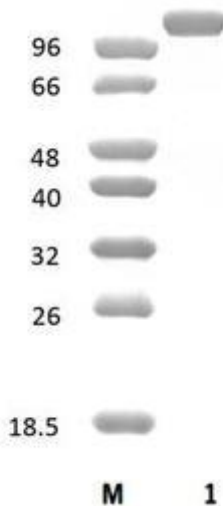
Figure 1. SDS-PAGE analysis of BtMns38A (GH38) was conducted in (Lane 1), employing a 14% polyacrylamide gel. The enzyme exhibits a band corresponding to a molecular weight of approximately 134,3 kDa. Lane M contains a Protein Marker for reference.
