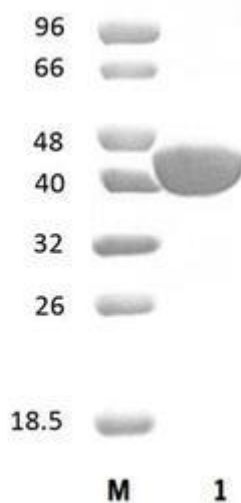
Figure 1. SDS-PAGE analysis of BtMan76A (GH76) was conducted in (Lane 1), employing a 14% polyacrylamide gel. The enzyme exhibits a band corresponding to a molecular weight of approximately 45,40 kDa. Lane M contains a Protein Marker for reference.
