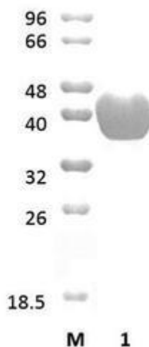
Figure 1. SDS-PAGE analysis of CtMan26C (GH26) was conducted in (Lane 1), employing a 14% polyacrylamide gel. The enzyme exhibits a band corresponding to a molecular weight of approximately 42,05 kDa. Lane M contains a Protein Marker for reference.
