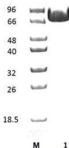
Figure 1. SDS-PAGE analysis of BtMns92H (GH92) was conducted in (Lane 1), employing a 14% polyacrylamide gel. The enzyme exhibits a band corresponding to a molecular weight of approximately 84,67 kDa. Lane M contains a Protein Marker for reference.
