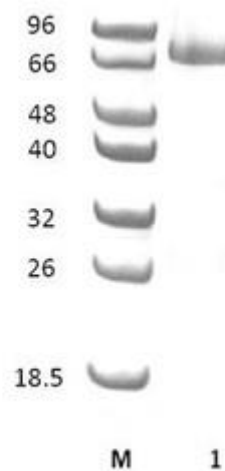
Figure 1. SDS-PAGE analysis of BtGal97A (GH97) was conducted in (Lane 1), employing a 14% polyacrylamide gel. The enzyme exhibits a band corresponding to a molecular weight of approximately 74,74 kDa. Lane M contains a Protein Marker for reference.
