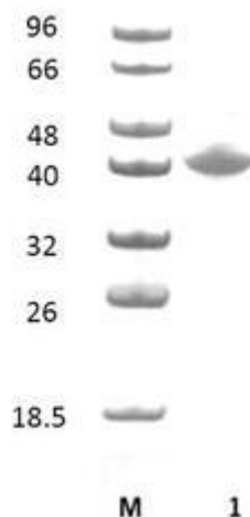
Figure 1. SDS-PAGE analysis of BtMns99B (GH99) was conducted in (Lane 1), employing a 14% polyacrylamide gel. The enzyme exhibits a band corresponding to a molecular weight of approximately 40,97 kDa. Lane M contains a Protein Marker for reference.
