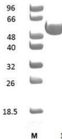
Figure 1. SDS-PAGE analysis of EcPbg1A (GH1) was conducted in (Lane 1), employing a 14% polyacrylamide gel. The enzyme exhibits a band corresponding to a molecular weight of approximately 57,16 kDa. Lane M contains a Protein Marker for reference.
