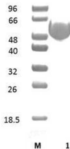
Figure 1. SDS-PAGE analysis of EcLaccA (AA NC) was conducted in (Lane 1), employing a 14% polyacrylamide gel. The enzyme exhibits a band corresponding to a molecular weight of approximately 55,47 kDa. Lane M contains a Protein Marker for reference.
