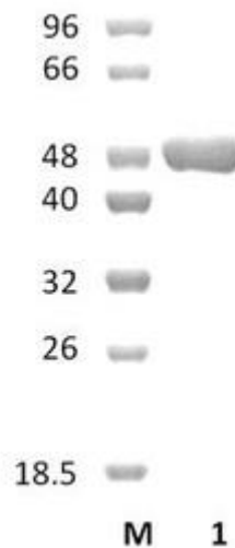
Figure 1. SDS-PAGE analysis of GFP-CBM27 was conducted in (Lane 1), employing a 14% polyacrylamide gel. The enzyme exhibits a band corresponding to a molecular weight of approximately 49,49 kDa. Lane M contains a Protein Marker for reference.
