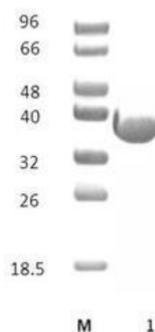
Figure 1. SDS-PAGE analysis of CtXyn10D (GH10) was conducted in (Lane 1), employing a 14% polyacrylamide gel. The enzyme exhibits a band corresponding to a molecular weight of approximately 39,56 kDa. Lane M contains a Protein Marker for reference.
