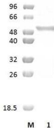
Figure 1. SDS-PAGE analysis of BtAbn43A (GH43) was conducted in (Lane 1), employing a 14% polyacrylamide gel. The enzyme exhibits a band corresponding to a molecular weight of approximately 56,86 kDa. Lane M contains a Protein Marker for reference.
