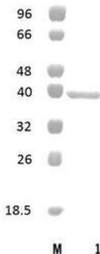
Figure 1. SDS-PAGE analysis of EcMlt102A (GH102) was conducted in (Lane 1), employing a 14% polyacrylamide gel. The enzyme exhibits a band corresponding to a molecular weight of approximately 38,34 kDa. Lane M contains a Protein Marker for reference.
