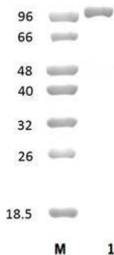
Figure 1. SDS-PAGE analysis of BtLac2A (GH2) was conducted in (Lane 1), employing a 14% polyacrylamide gel. The enzyme exhibits a band corresponding to a molecular weight of approximately 108,4 kDa. Lane M contains a Protein Marker for reference.
