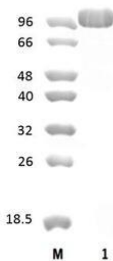
Figure 1. SDS-PAGE analysis of BtMan76B (GH76) was conducted in (Lane 1), employing a 14% polyacrylamide gel. The enzyme exhibits a band corresponding to a molecular weight of approximately 100,4 kDa. Lane M contains a Protein Marker for reference.
