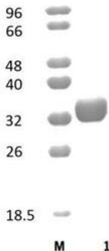
Figure 1. SDS-PAGE analysis of CpGng16C (GH16) was conducted in (Lane 1), employing a 14% polyacrylamide gel. The enzyme exhibits a band corresponding to a molecular weight of approximately 33,73 kDa. Lane M contains a Protein Marker for reference.
