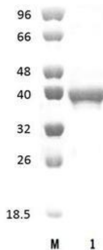
Figure 1. SDS-PAGE analysis of RfBgc5A (GH5) was conducted in (Lane 1), employing a 14% polyacrylamide gel. The enzyme exhibits a band corresponding to a molecular weight of approximately 38,81 kDa. Lane M contains a Protein Marker for reference.
