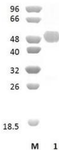
Figure 1. SDS-PAGE analysis of DdPgl28A (GH28) was conducted in (Lane 1), employing a 14% polyacrylamide gel. The enzyme exhibits a band corresponding to a molecular weight of approximately 48,67 kDa. Lane M contains a Protein Marker for reference.
