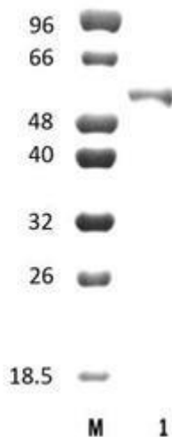
Figure 1. SDS-PAGE analysis of SmPbg1A (GH1) was conducted in (Lane 1), employing a 14% polyacrylamide gel. The enzyme exhibits a band corresponding to a molecular weight of approximately 56,42 kDa. Lane M contains a Protein Marker for reference.
