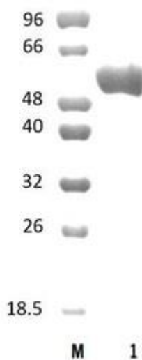
Figure 1. SDS-PAGE analysis of SmPbg1B (GH1) was conducted in (Lane 1), employing a 14% polyacrylamide gel. The enzyme exhibits a band corresponding to a molecular weight of approximately 57,20 kDa. Lane M contains a Protein Marker for reference.
