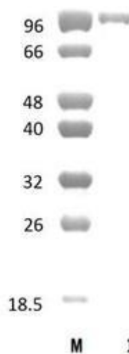
Figure 1. SDS-PAGE analysis of SmGtf70C (GH70) was conducted in (Lane 1), employing a 14% polyacrylamide gel. The enzyme exhibits a band corresponding to a molecular weight of approximately 98,96 kDa. Lane M contains a Protein Marker for reference.
