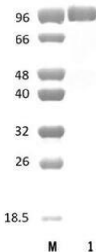
Figure 1. SDS-PAGE analysis of SmGtf70D (GH70) was conducted in (Lane 1), employing a 14% polyacrylamide gel. The enzyme exhibits a band corresponding to a molecular weight of approximately 98,48 kDa. Lane M contains a Protein Marker for reference.
