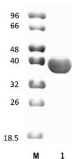
Figure 1. SDS-PAGE analysis of TfXyn10A (GH10) was conducted in (Lane 1), employing a 14% polyacrylamide gel. The enzyme exhibits a band corresponding to a molecular weight of approximately 40,68 kDa. Lane M contains a Protein Marker for reference.
