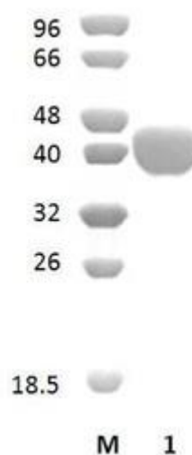
Figure 1. SDS-PAGE analysis of SpHex20A (GH20) was conducted in (Lane 1), employing a 14% polyacrylamide gel. The enzyme exhibits a band corresponding to a molecular weight of approximately 43,11 kDa. Lane M contains a Protein Marker for reference.
