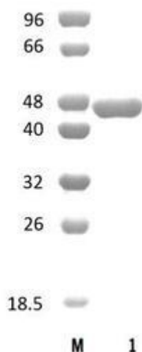
Figure 1. SDS-PAGE analysis of B/Gan53A (GH53) was conducted in (Lane 1), employing a 14% polyacrylamide gel. The enzyme exhibits a band corresponding to a molecular weight of approximately 45,68 kDa. Lane M contains a Protein Marker for reference.
