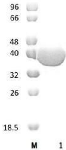
Figure 1. SDS-PAGE analysis of SdHex3C (GH3) was conducted in (Lane 1), employing a 14% polyacrylamide gel. The enzyme exhibits a band corresponding to a molecular weight of approximately 39,56 kDa. Lane M contains a Protein Marker for reference.
