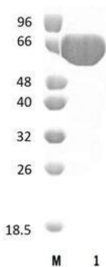
Figure 1. SDS-PAGE analysis of BcAgl13A (GH13) was conducted in (Lane 1), employing a 14% polyacrylamide gel. The enzyme exhibits a band corresponding to a molecular weight of approximately 67,86 kDa. Lane M contains a Protein Marker for reference.
