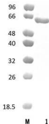
Figure 1. SDS-PAGE analysis of PfMns1A (GH1) was conducted in (Lane 1), employing a 14% polyacrylamide gel. The enzyme exhibits a band corresponding to a molecular weight of approximately 61,16 kDa. Lane M contains a Protein Marker for reference.
