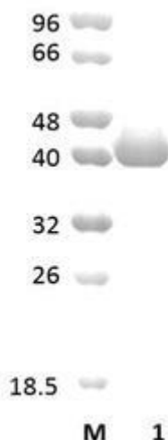
Figure 1. SDS-PAGE analysis of GFP-CBM62 was conducted in (Lane 1), employing a 14% polyacrylamide gel. The enzyme exhibits a band corresponding to a molecular weight of approximately 44,43 kDa. Lane M contains a Protein Marker for reference.
