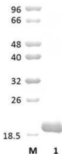
Figure 1. SDS-PAGE analysis of CBM4 was conducted in (Lane 1), employing a 14% polyacrylamide gel. The enzyme exhibits a band corresponding to a molecular weight of approximately 19,72 kDa. Lane M contains a Protein Marker for reference.
