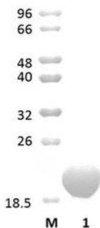
Figure 1. SDS-PAGE analysis of CBM22 was conducted in (Lane 1), employing a 14% polyacrylamide gel. The enzyme exhibits a band corresponding to a molecular weight of approximately 19,65 kDa. Lane M contains a Protein Marker for reference.
