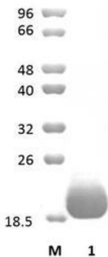
Figure 1. SDS-PAGE analysis of CBM22 was conducted in (Lane 1), employing a 14% polyacrylamide gel. The enzyme exhibits a band corresponding to a molecular weight of approximately 19,57 kDa. Lane M contains a Protein Marker for reference.
