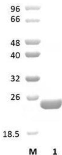
Figure 1. SDS-PAGE analysis of CBM22 was conducted in (Lane 1), employing a 14% polyacrylamide gel. The enzyme exhibits a band corresponding to a molecular weight of approximately 17,89 kDa. Lane M contains a Protein Marker for reference.
