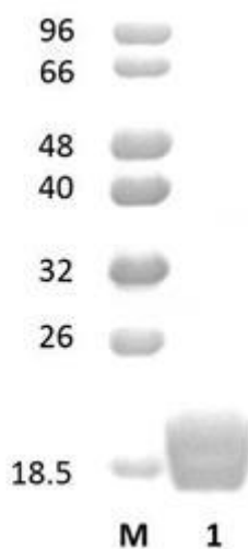
Figure 1. SDS-PAGE analysis of CBM13 was conducted in (Lane 1), employing a 14% polyacrylamide gel. The enzyme exhibits a band corresponding to a molecular weight of approximately 18,47 kDa. Lane M contains a Protein Marker for reference.
