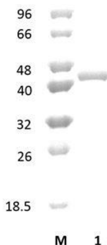
Figure 1. SDS-PAGE analysis of CsXyn10A (GH10) was conducted in (Lane 1), employing a 14% polyacrylamide gel. The enzyme exhibits a band corresponding to a molecular weight of approximately 42,55 kDa. Lane M contains a Protein Marker for reference.
