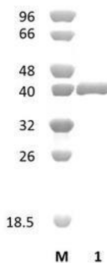
Figure 1. SDS-PAGE analysis of PpMan26A (GH26) was conducted in (Lane 1), employing a 14% polyacrylamide gel. The enzyme exhibits a band corresponding to a molecular weight of approximately 37,61 kDa. Lane M contains a Protein Marker for reference.
