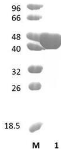
Figure 1. SDS-PAGE analysis of BcCsn8B (GH8) was conducted in (Lane 1), employing a 14% polyacrylamide gel. The enzyme exhibits a band corresponding to a molecular weight of approximately 47,88 kDa. Lane M contains a Protein Marker for reference.
