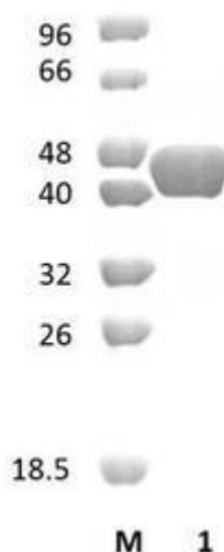
Figure 1. SDS-PAGE analysis of TpMan5A (GH5) was conducted in (Lane 1), employing a 14% polyacrylamide gel. The enzyme exhibits a band corresponding to a molecular weight of approximately 46,16 kDa. Lane M contains a Protein Marker for reference.
