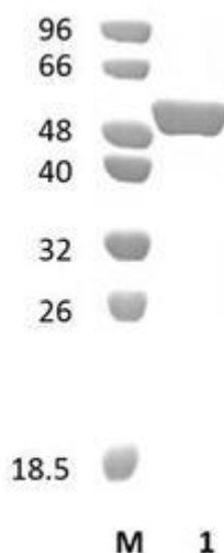
Figure 1. SDS-PAGE analysis of CcBgl1A (GH1) was conducted in (Lane 1), employing a 14% polyacrylamide gel. The enzyme exhibits a band corresponding to a molecular weight of approximately 53,66 kDa. Lane M contains a Protein Marker for reference.
