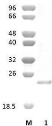
Figure 1. SDS-PAGE analysis of L/Lpmo10A (AA10) was conducted in (Lane 1), employing a 14% polyacrylamide gel. The enzyme exhibits a band corresponding to a molecular weight of approximately 20,89 kDa. Lane M contains a Protein Marker for reference.
